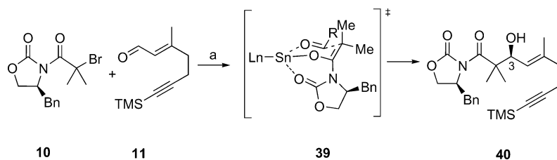
Scheme 9. Reformatsky reaction. Reagents and conditions: (a) (i) \text{SnCl}_2 , \text{LiAlH}_4 , THF, 23 °C; (ii) 10 , –78 °C; (iii) 11 , –78 °C, 78%.
