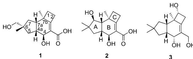
Figure 1. Pasteurestin A ( 1 ), pasteurestin B ( 2 ), and illudol ( 3 ).
