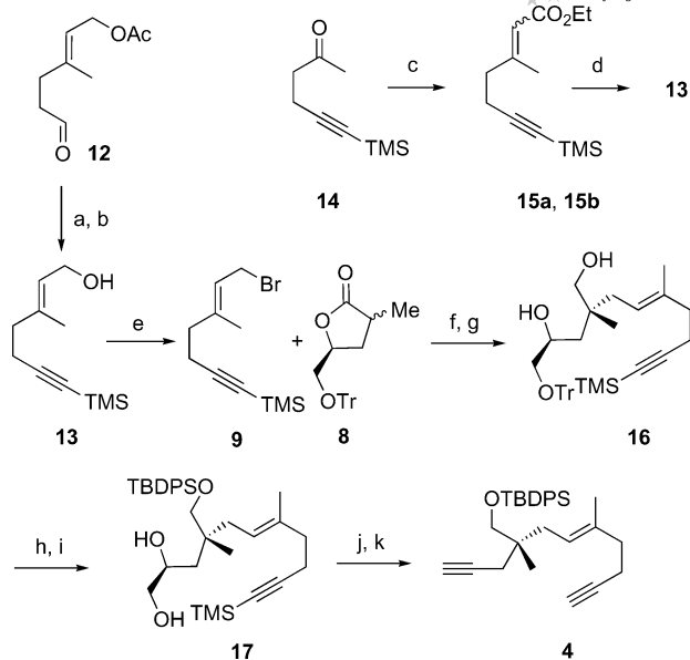
Scheme 3. Synthesis of enediyne 4 . Reagents and conditions: (a) \text{K}_2\text{CO}_3 , (\text{MeO})_2\text{P}(\text{O})\text{CN}_2\text{C}(\text{O})\text{Me} , MeOH, 23 °C, 90%; (b) (i) n BuLi, TMSCl, THF, –78 °C, (ii) HCl 2 N, 23 °C, 95%; (c) NaH, (\text{EtO})_2\text{P}(\text{O})\text{CH}_2\text{CO}_2\text{Et} , THF, 72%; (d) DIBAL-H, THF, –78 °C, 90%; (e) \text{CBr}_4 , \text{PPh}_3 , \text{CH}_2\text{Cl}_2 , 0 °C, 84%; (f) 8 , LDA, HMPA, THF, –78 °C, then 9 , 71%; (g) DIBAL-H, THF, –78 °C, 95%; (h) TBDPSCl, DMAP, \text{NEt}_3 , \text{CH}_2\text{Cl}_2 , 23 °C, 90%; (i) \text{Et}_2\text{AlCl} , \text{CH}_2\text{Cl}_2 , –78 °C, 87%; (j) \text{Pb}(\text{OAc})_4 , \text{CH}_2\text{Cl}_2 , 23 °C, 95%; (k) \text{K}_2\text{CO}_3 , MeOH, (\text{MeO})_2\text{P}(\text{O})\text{CN}_2\text{C}(\text{O})\text{Me} , 23 °C, 71%. HMPA = hexamethyl phosphoramide; LDA = lithium diisopropylamide; DIBAL-H = diisobutylaluminium hydride.
