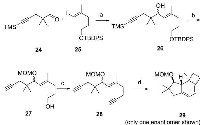
Scheme 7. Cyclotrimerization of test substrate 28 . Reagents and conditions: (a) 25 , t BuLi, -78^{\circ}\text{C} to 0^{\circ}\text{C} , then 24 , -78^{\circ}\text{C} to room temp., 56%; (b) (i) MOMCl, DIPEA, CH 2 Cl 2 , (ii) TBAF, THF, 80%; (c) (i) DMP, CH 2 Cl 2 , room temp., (ii) K 2 CO 3 , MeOH, (MeO) 2 P(O)CN 2 C(O)Me, 23^{\circ}\text{C} , 92%; (d) CoCp(CO) 2 , toluene, reflux, then CuCl 2 ·2H 2 O, DME, 23^{\circ}\text{C} , 43%. MOM = methoxymethyl; DIPEA = diisopropylethylamine.
