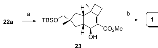
Scheme 6. Endgame in the synthesis of pasteurin A ( 1 ). Reagents and conditions: (a) \text{NaBH}_4 , \text{CeCl}_3 \cdot 7\text{H}_2\text{O} , MeOH, 87%; (b) (i) HF·Py, THF, 23 °C; (ii) LiOH, \text{H}_2\text{O}/\text{THF} , 23 °C, 55%. Py = pyridine.
