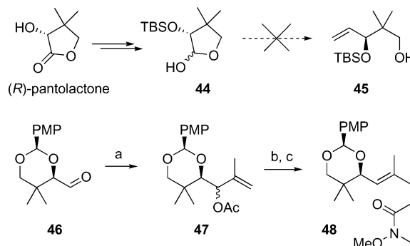
Scheme 11. Pantolactone approach. Reagents and conditions: (a) (i) isopropenylMgBr, THF, 0 °C; (ii) \text{Ac}_2\text{O} , \text{NEt}_3 , DMAP, \text{CH}_2\text{Cl}_2 , 23 °C, 80%; (b) LDA, TMSCl, –78 °C to 23 °C, 69%; (c) DIC, \text{NEt}_3 , MeHNOMe·HCl, \text{CH}_2\text{Cl}_2 , 23 °C, 98%. DMAP = 4-(dimethylamino)pyridine; LDA = lithium diisopropylamide; DIC = N,N' -diisopropylcarbodiimide; PMP = p -methoxyphenyl.
