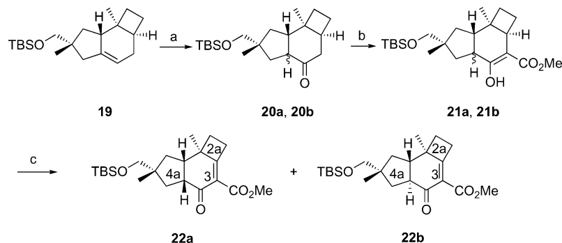
Scheme 5. Functionalization of the six-membered ring. Reagents and conditions: (a) (i) \text{BH}_3 , THF, 23 °C, then \text{K}_2\text{CO}_3 , \text{H}_2\text{O}_2 , reflux, (ii) DMP, \text{CH}_2\text{Cl}_2 , 23 °C, 74%; (b) LDA, HMPA, THF, –78 °C, then \text{CO}_2 (excess), –58 °C, then 1 N HCl, 23 °C, then \text{TMSCHN}_2 , 0 °C, 55%, 75% (based on recovered starting material); (c) (i) LDA, PhSeCl, THF, –78 °C, (ii) \text{NH}_4\text{Cl} , \text{H}_2\text{O}_2 , \text{H}_2\text{O}/\text{CH}_2\text{Cl}_2 , 0 °C, 50%. DMP = Dess–Martin periodinane.
