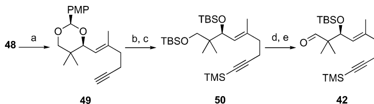
Scheme 12. Pantolactone approach II. Reagents and conditions: (a) (i) DIBAL-H, THF, -78^{\circ}\text{C} , 95%; (ii) TMSCHN 2 , n BuLi, THF, -78^{\circ}\text{C} , 67%; (b) n BuLi, TMSCl, THF, -78^{\circ}\text{C} , 95%; (c) (i) 80% AcOH, THF, (ii) TBSOTf, 2,6-lutidine, CH 2 Cl 2 , 0^{\circ}\text{C} , 91%; (d) HF·Py, THF, 23^{\circ}\text{C} , 65%; (e) DMP, CH 2 Cl 2 , 23^{\circ}\text{C} , 92%.
