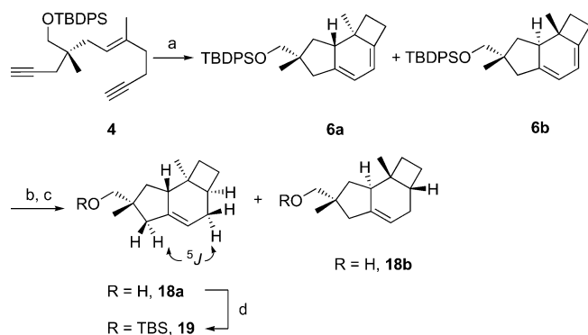
Scheme 4. [2+2+2] Cycloaddition and functionalization of dienes 6a and 6b . Reagents and conditions: (a) \text{CoCp}(\text{CO})_2 , toluene, reflux, then \text{CuCl}_2 \cdot 2\text{H}_2\text{O} , DME, 23 °C, 46%; (b) Li (excess), \text{NH}_3 , t BuOH, THF, –78 °C, 85%; (c) TBAF, THF, 23 °C, 95%; HPLC separation; (d) TBSCl, imidazole, DMF, 23 °C, 90%. Cp = cyclopentadienyl; DME = 1,2-dimethoxyethane; TBAF = tetrabutylammonium fluoride.
