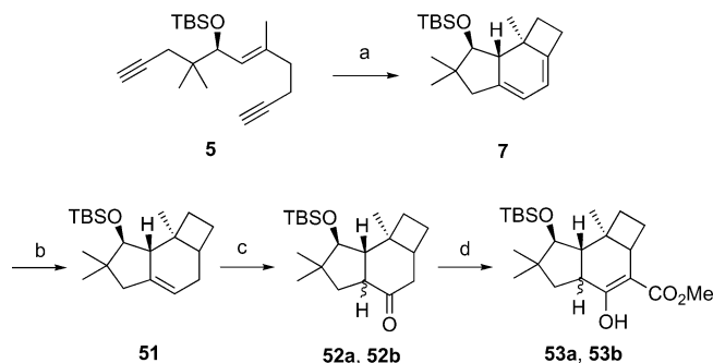
Scheme 13. [2+2+2] cycloaddition and functionalization of diene 7 . Reagents and conditions: (a) CoCp(CO) 2 , toluene, reflux, then CuCl 2 ·2H 2 O, DME, 23^{\circ}\text{C} , 40%; (b) Li (excess), NH 3 , t BuOH, THF, -78^{\circ}\text{C} , 85%; (c) (i) BH 3 , THF, 23^{\circ}\text{C} , then K 2 CO 3 , H 2 O 2 , THF/H 2 O, reflux, (ii) DMP, CH 2 Cl 2 , 23^{\circ}\text{C} , 74%; (d) LDA, HMPA, THF, -78^{\circ}\text{C} , then CO 2 (excess), -58^{\circ}\text{C} , then 1 N HCl, 23^{\circ}\text{C} , then TMSCHN 2 , 0^{\circ}\text{C} , 45%, 75% (based on recovered starting material); (e) (i) LDA, PhSeCl, THF, -78^{\circ}\text{C} , (ii) NH 4 Cl, H 2 O 2 , H 2 O/CH 2 Cl 2 , 0^{\circ}\text{C} , 45%.
