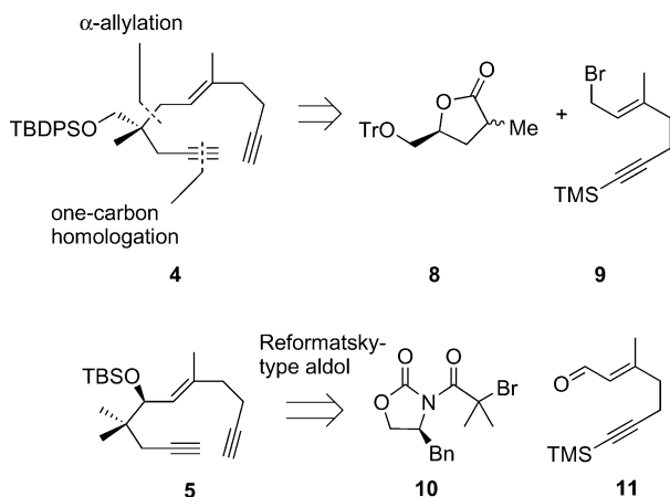
Scheme 2. Retrosynthetic analysis for enediynes 4 and 5 . Tr = triphenylmethyl; TMS = trimethylsilyl.
