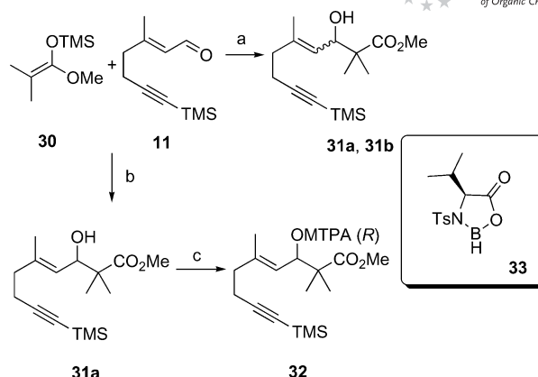
Scheme 8. Mukaiyama aldol reaction. Reagents and conditions: (a) (i) 33 , THF, DCM, room temp., (ii) 11 , DCM, -78^{\circ}\text{C} , (iii) 30 , DCM, -78^{\circ}\text{C} , 89%; (b) (i) 11 , 30 , DCM, -78^{\circ}\text{C} , (ii) 33 , DCM, room temp., 75%; (c) ( S )-Mosher's acyl chloride, pyridine, DCM, 0^{\circ}\text{C} , 70%. Ts = p -toluenesulfonate.
