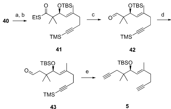
Scheme 10. Synthesis of the enediyne 5 . Reagents and conditions: (a) TBSOTf, 2,6-lutidine, \text{CH}_2\text{Cl}_2 , 0 °C, 95%; (b) n\text{BuLi} , EtSH, THF, 0 °C, 89%; (c) DIBAL-H, \text{CH}_2\text{Cl}_2 , –78 °C, 75% (+15% alcohol); (d) \text{MeOCH}_2\text{PPh}_3\text{Cl} , n\text{BuLi} , 0 °C, then HCl 2 M, 23 °C, 60%; (e) \text{K}_2\text{CO}_3 , (\text{MeO})_2\text{P}(\text{O})\text{CN}_2\text{C}(\text{O})\text{Me} , MeOH, 23 °C, 94%. Tf = trifluoromethanesulfonate.
