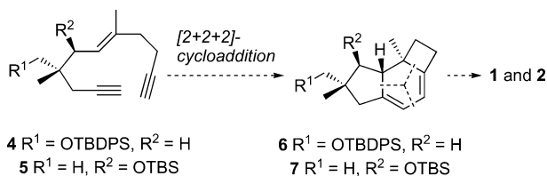
Scheme 1. Synthetic plan for pasteurestins A ( 1 ) and B ( 2 ). TBDPS = tert -butyldiphenylsilyl; TBS = tert -butyldimethylsilyl.
